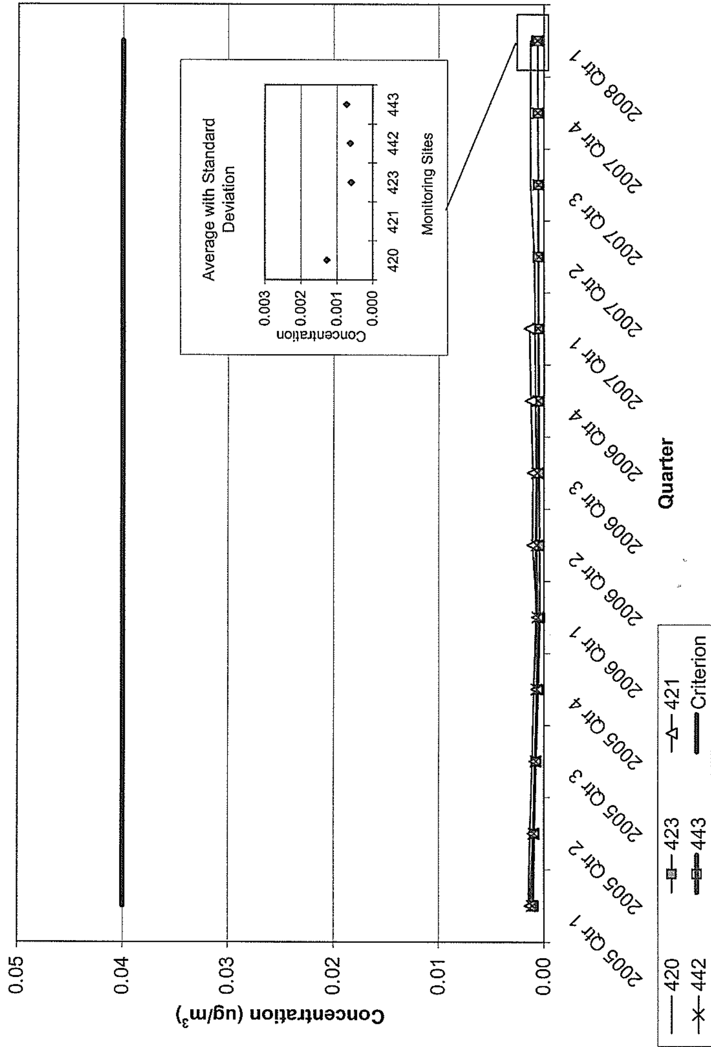
Figure 17 Nickel Annual Average Concentration
